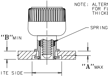
UNFASTENED PART NUMBER: 47-10-2X1-YO SHOWN
