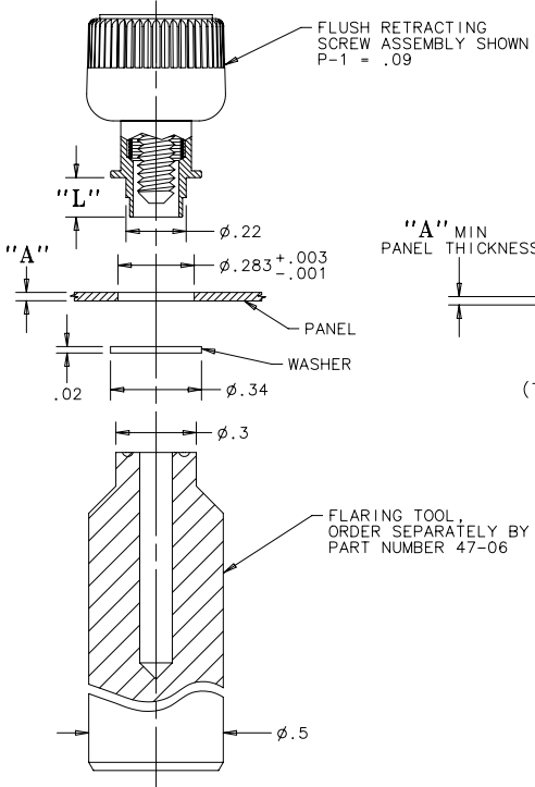
PANEL PREPARATION PART NUMBER: 47-10-2X1-YO SHOWN
