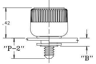
FASTENED PART NUMBER: 47-10-2X1-YO SHOWN
