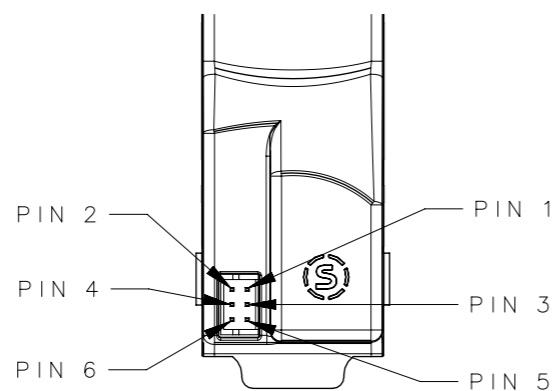
ACTUATOR PIN-OUT DIAGRAM (SEE NOTE D)
