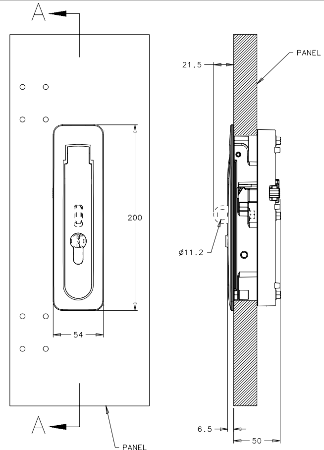
SECTION A-A PANEL SECTIONED ONLY
