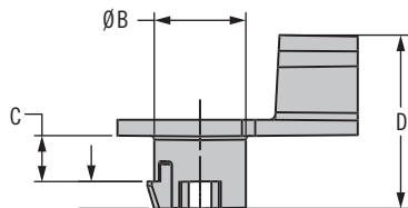
Slotted hole trigger / lever (R4-0-72894-X)
