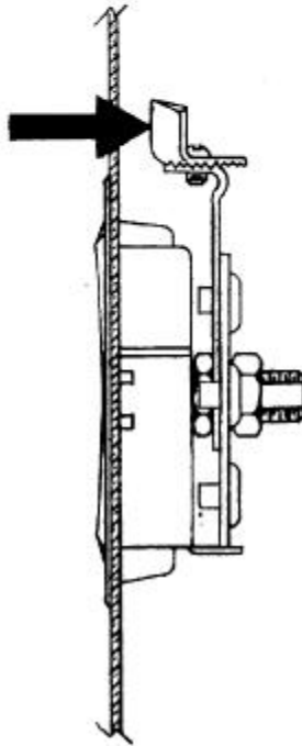
N° 01 RECESSED CUP LATCH PART N° 01-10-401-10
