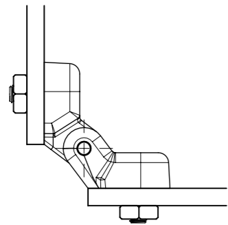
RADIAL @ 90°
