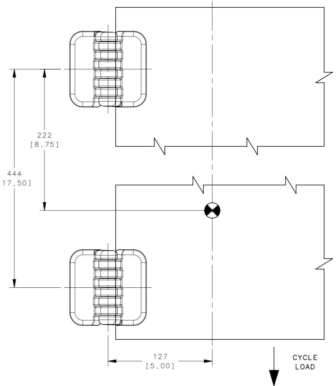
CYCLE TEST SET-UP
