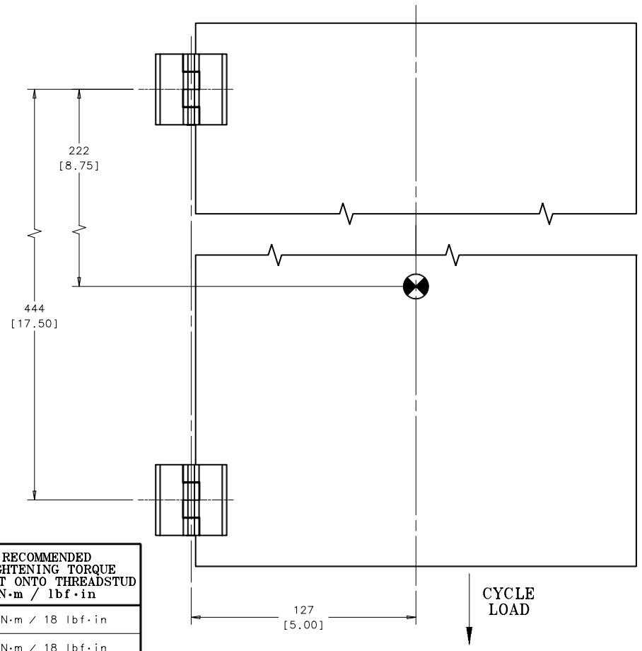
CYCLE TEST SET-UP (SCALE .5:1)
