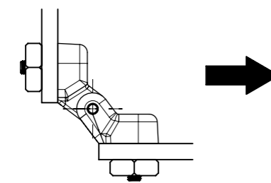
RADIAL @ 90°
