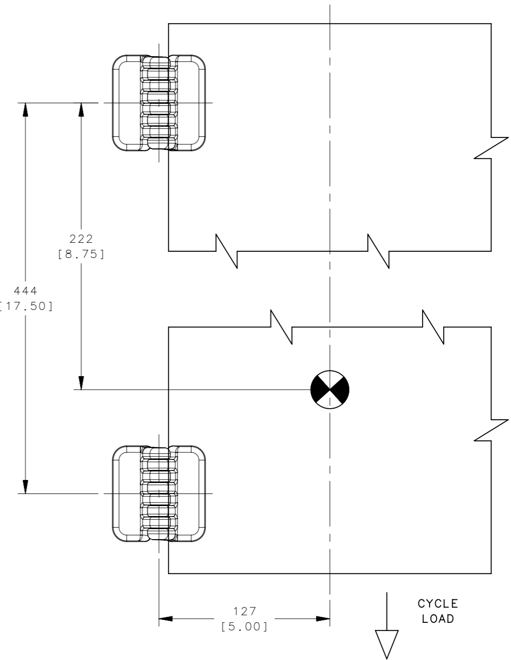
CYCLE TEST SET-UP
