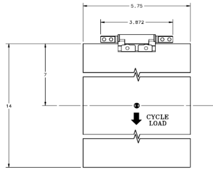
CYCLE TEST SET-UP SCALE .50:1 PANEL WEIGHT: 6.49 lb
