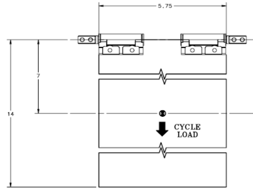
CYCLE TEST SET-UP SCALE .50:1 PANEL WEIGHT: 6.58 lb.
